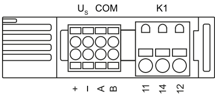
Figure 4-2: isoGEN413R-1 bottom
