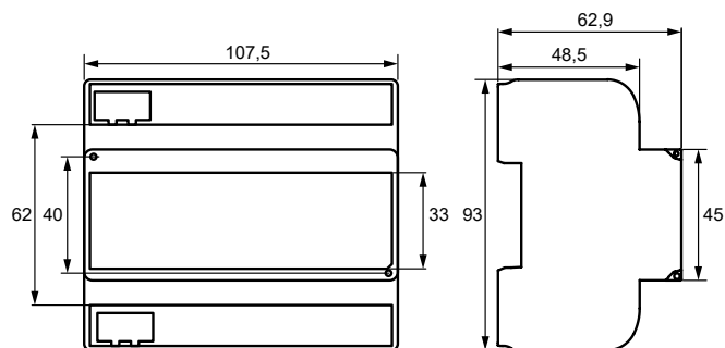
Dimension diagram (in mm)
